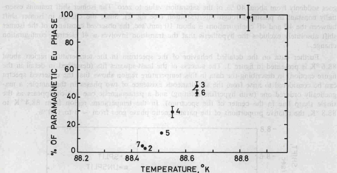
Fig. 5. — Ratio of the areas of the ordered and paramagnetic parts of the absorption spectra in the transition region. The points are numbered in the order in which the runs were made. The figure shows clearly the absence of hysteresis. The total transition width is about 0.3 °K. The transition width and temperature appear to lie intermediate between those for the two samples used in Ref. 2.
