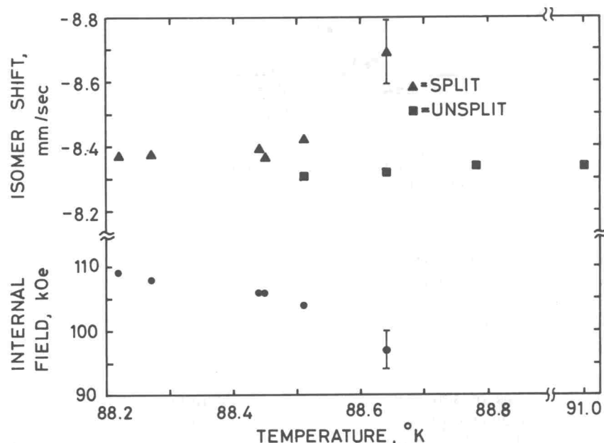
FIG. 4. — Internal fields and isomer shifts obtained from the least-squares fits shown in Figure 3. Error bars shown are 1\sigma ; where no errors are indicated, they are about the size of the points. Note that the H_{int} of the split spectrum changes only very slightly in the transition region.
